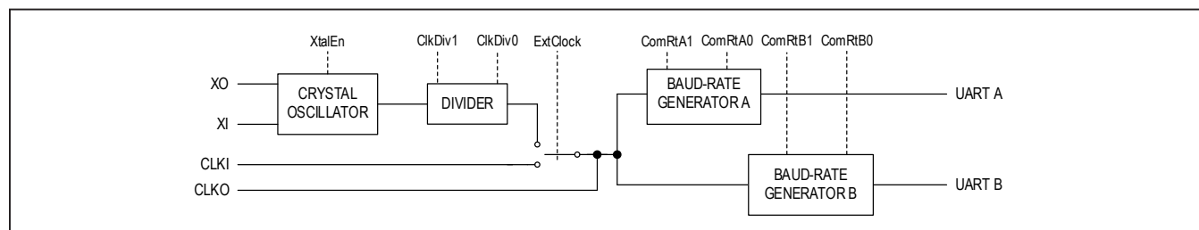
Figure 15. Clock Generation
